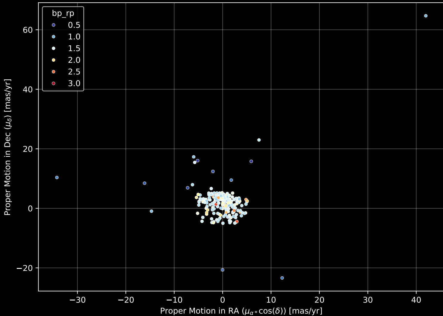
APOGEE DR17 Field: [291-25-C] Proper Motion Diagram (n= 224)
