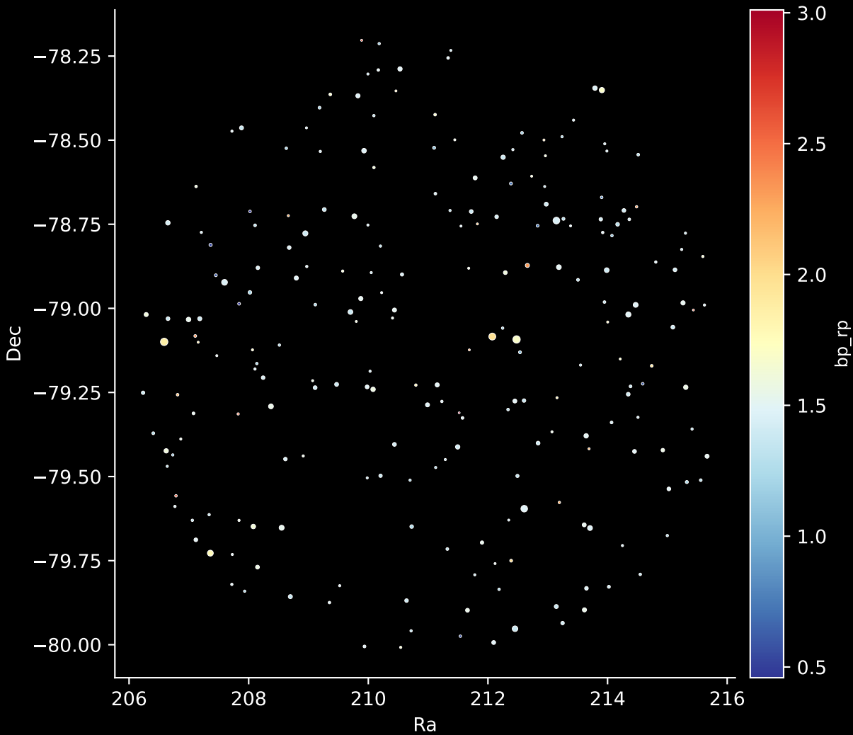
APOGEE DR17 Field: [291-25-C] Stars: 224
