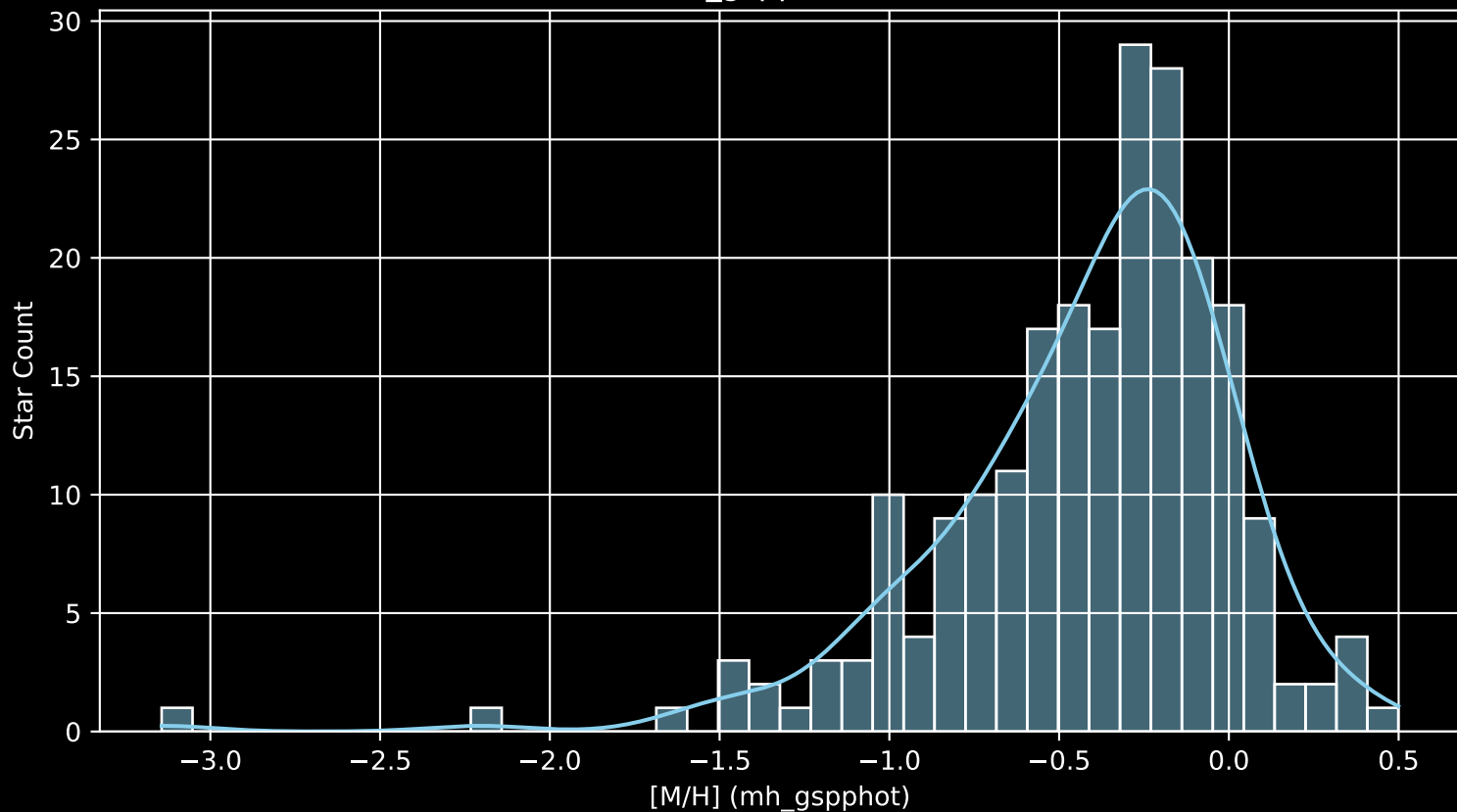
APOGEE DR17 Field: [291-25-C [M/H] (mh_gspphot) (n= 224)
