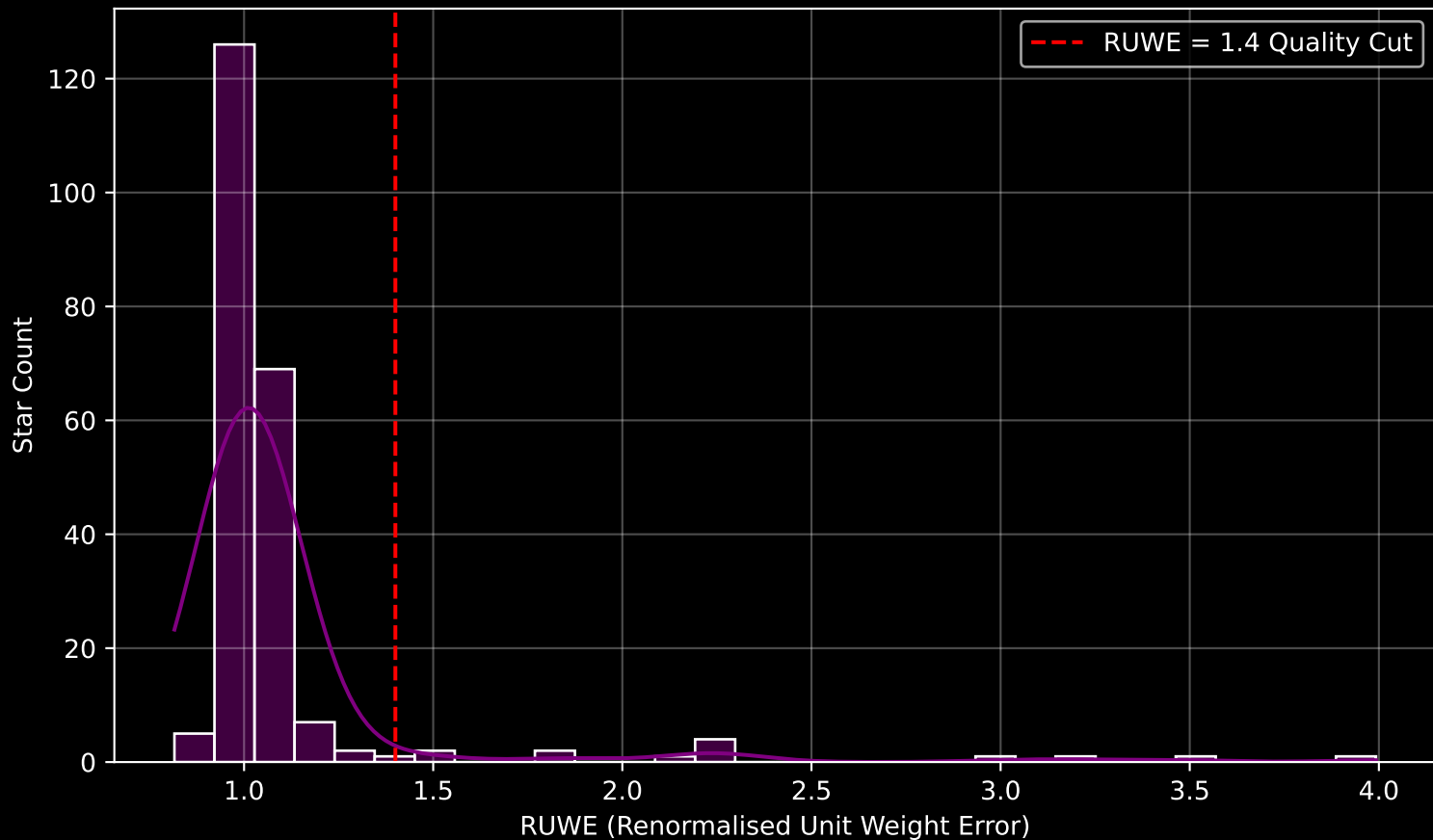
GAPOGEE DR17 Field [291-25-C] RUWE Distribution (n= 223)
