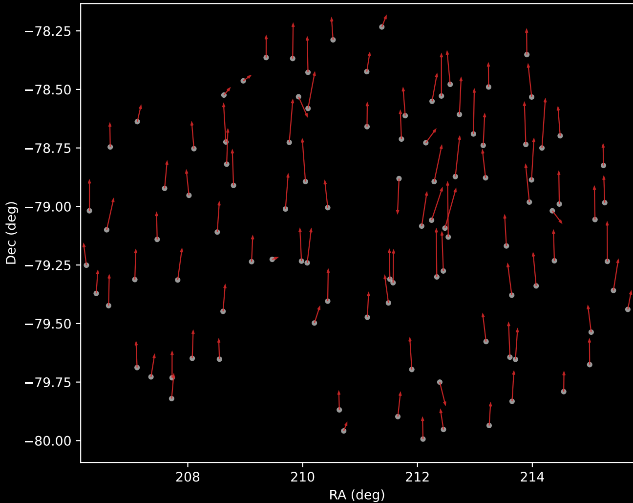
APOGEE DR17 Cluster 6 Proper Motion Vectors (n=103)
