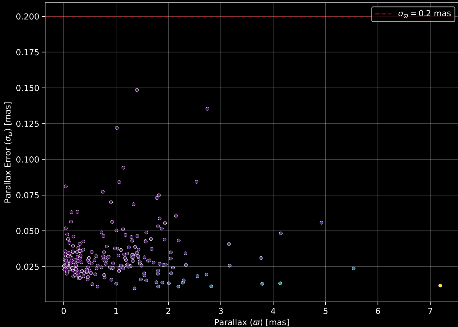
APOGEE DR17 Field: [291-25-C] Parallax Quality (n= 224)
