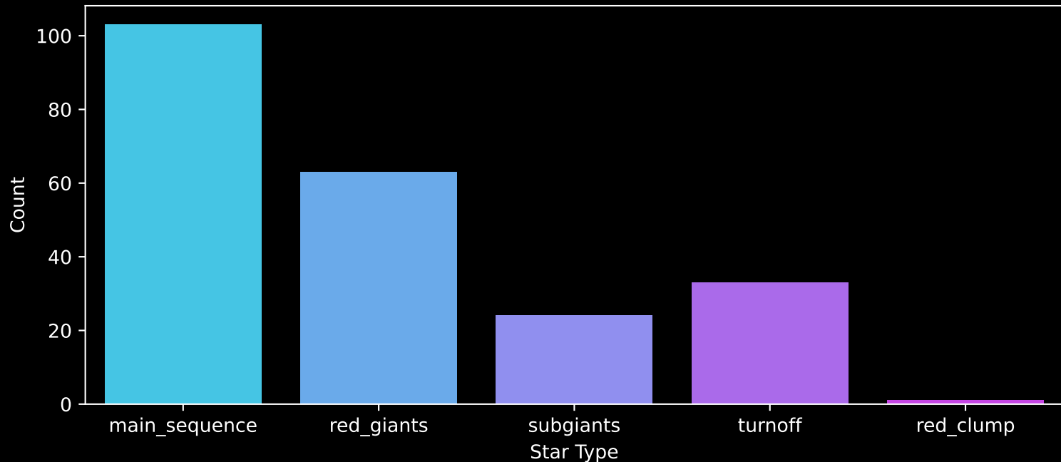
APOGEE DR17 Field: [291-25-C] Count plot of Star Type
